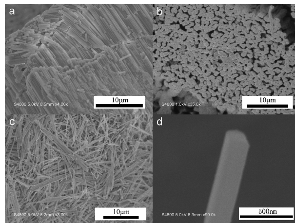
Figure 1. FE-SEM images of the prepared nanorod arrays (a), (b) and separate nanorods (c), (d).
