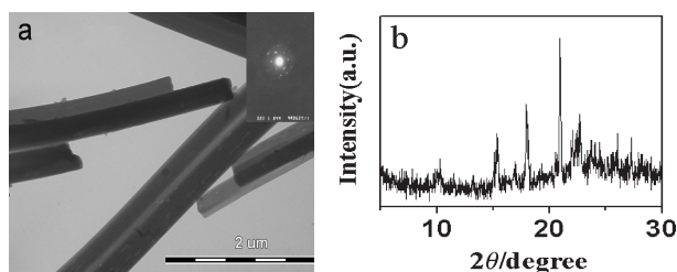
Figure 2. TEM image (a) and XRD pattern (b) of ZnQ 2 nanorods, insert is SAED pattern.
