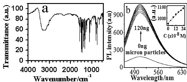
Figure 3. (a) IR spectrum of ZnQ 2 nanorods, (b) PL spectra of ZnQ 2 submicron particles, and nanorods mixed with different concentration of aqueous melamine solution. Insert is the linearity curve of PL intensities vs. the concentrations of melamine mixed with ZnQ 2 nanorods.
